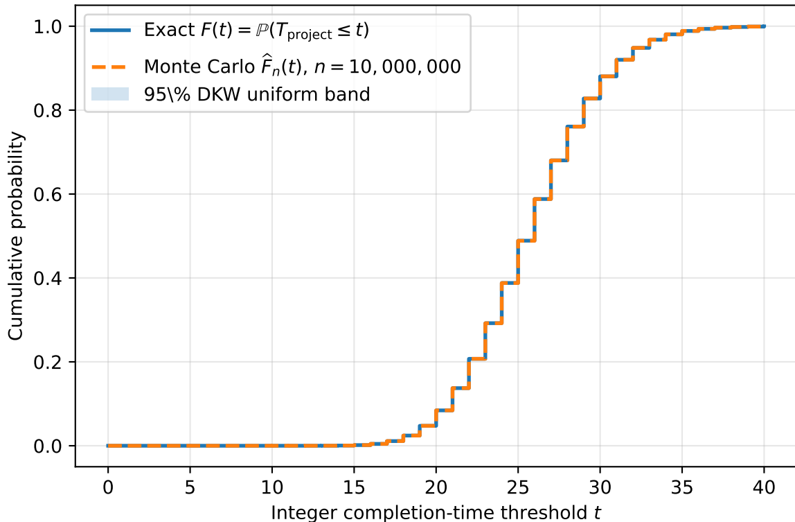
Exact discrete CDF versus Monte Carlo empirical CDF
